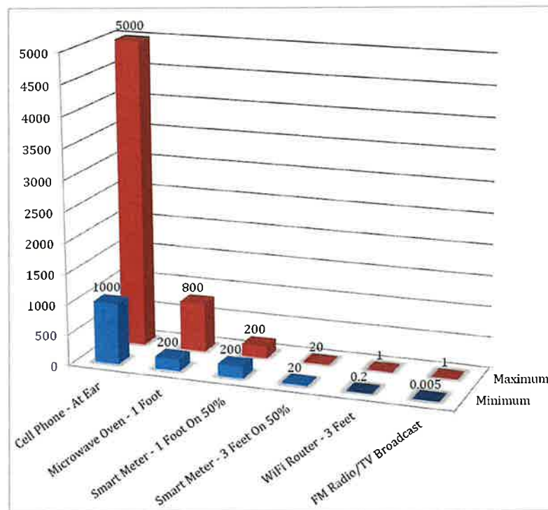
Figure 1: Comparison of Radio-Frequency Levels from Various Sources (in \mu\text{W}/\text{cm}^2 )
