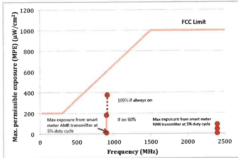
Figure 3: FCC Maximum Exposure Limits and Exposure from a 900 MHz, 1 Watt smart meter 1 foot from the user
